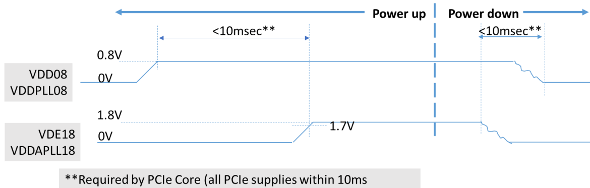
Figure 17: Power Sequence Diagram
