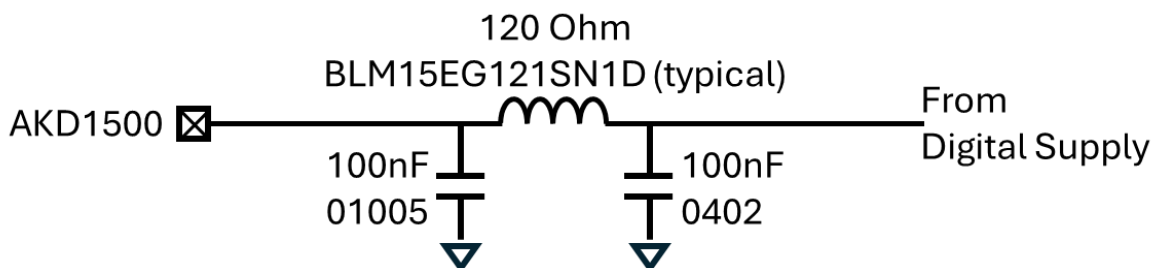
Figure 18: Filtering analog supply lines
